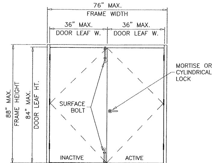
DOUBLE OUTSWING STEEL DOOR UNDER SEPARATE APPROVAL
