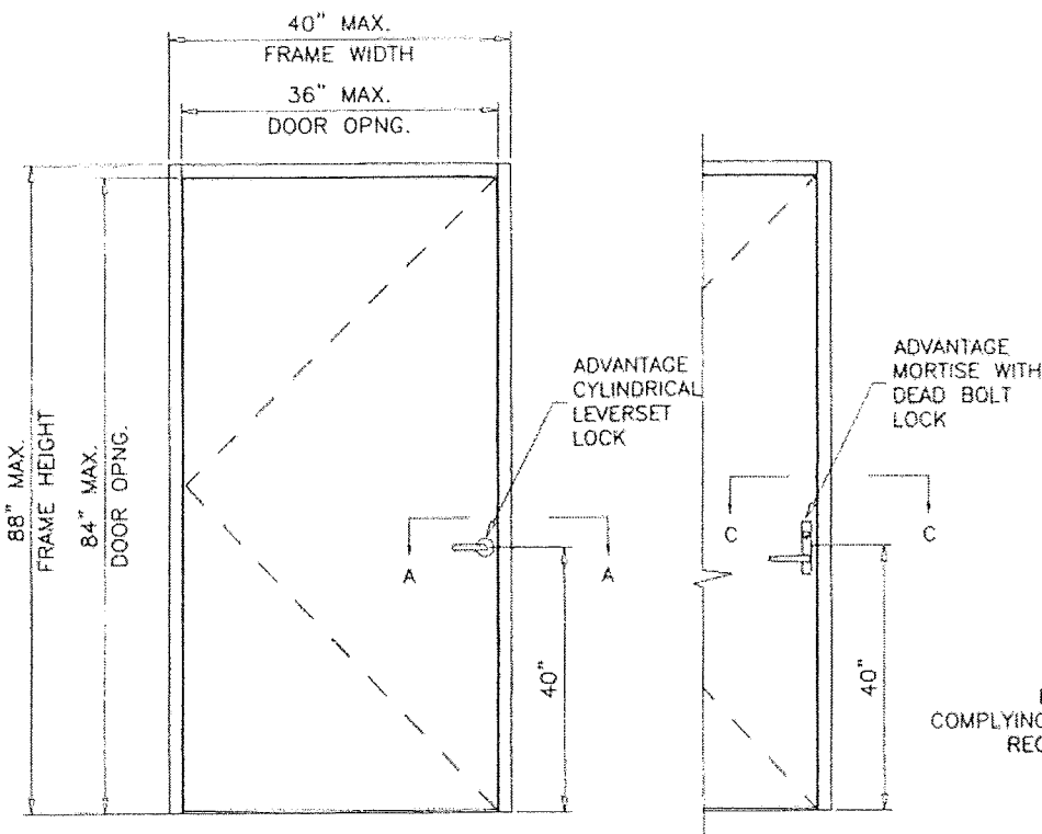
SINGLE OUTSWING STEEL DOOR UNDER SEPARATE APPROVAL
